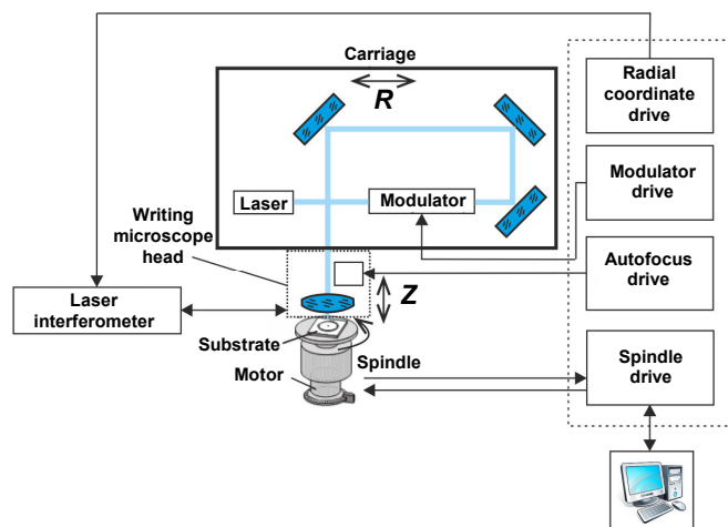
Fig.14. Structure scheme of laser image generator using semiconductor laser.
