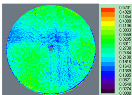
Fig.16. Report summary (from Intellium Z100 interferometer) and wavefront distortion map for the diffractive lens manufactured by the updated laser image generator.
