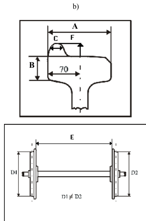
Fig.6. The principle of self-scanning for the running freight car wheels using triangulation measuring sensors (a) and wheel parameters under inspection. (b).
