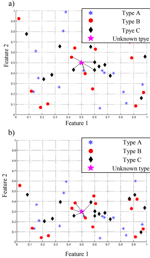
Fig.1. Vector space (a) w=[1,1] , (b) w=[1,0.6] .
