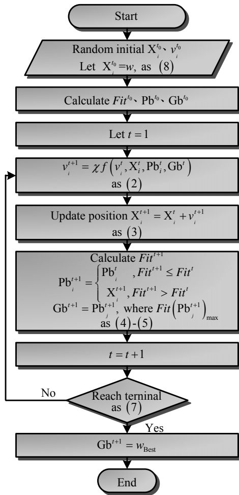
Fig.2. PWKNN flowchart.
