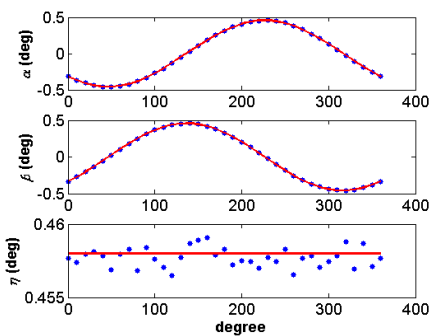
Fig.17. One-circle measurement.
