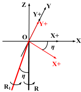
Fig.2. Using an inclinometer to measure rotating shaft tilt angle.
