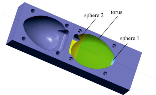
Fig.1. Complex workpiece surface separated into geometric features.
