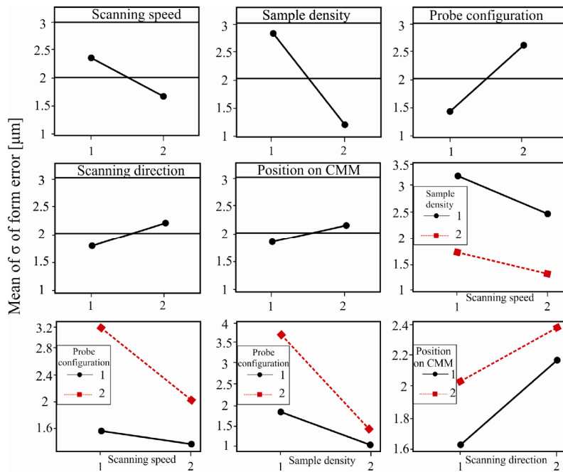
Fig.3. Main Effects Plot and Interaction Plot(data means) for \sigma of form error [ \mu\text{m} ].
