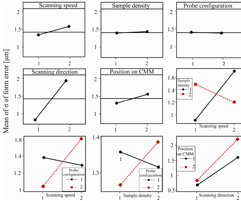
Fig.2. Effect of individual factors and their interactions on the standard deviation in the measurement of the torus.
