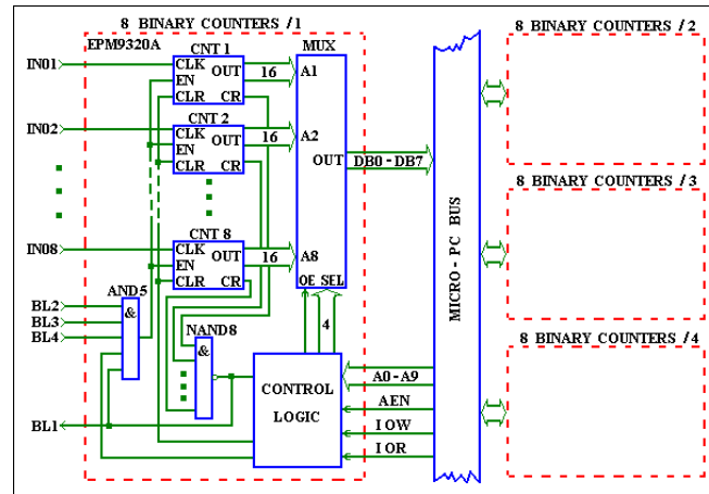
Fig. 3. Structural layout of counters module
