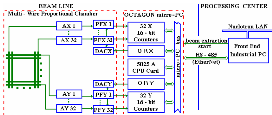
Fig. 1. Structural layout of profilometer based on MWPC use
