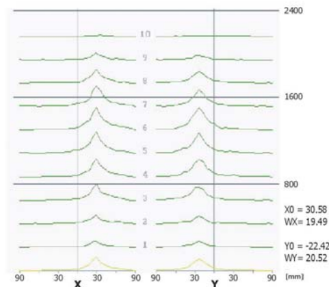
Fig. 6. Representation of the data measured in the multiple reading mode
