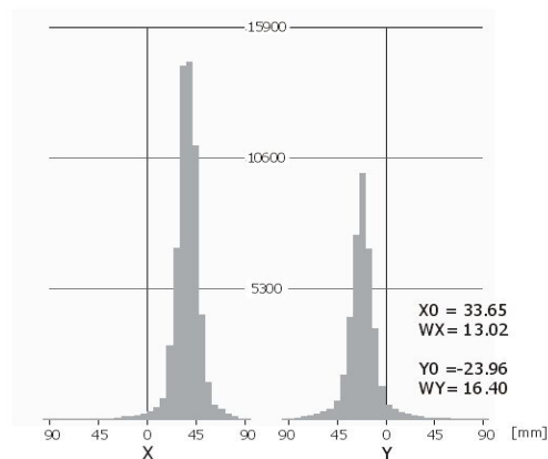
Fig. 5. Integral beam profiles
