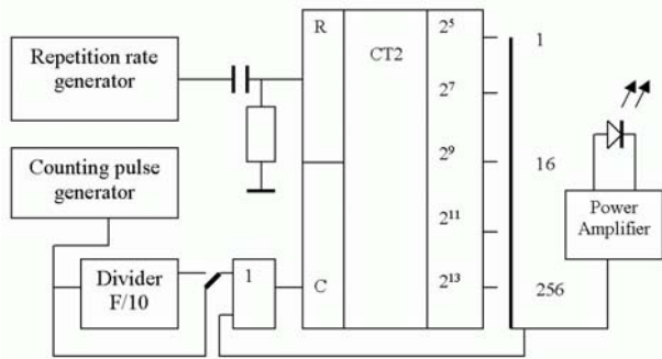
Fig.3 Schematic diagram of experimental unit.
