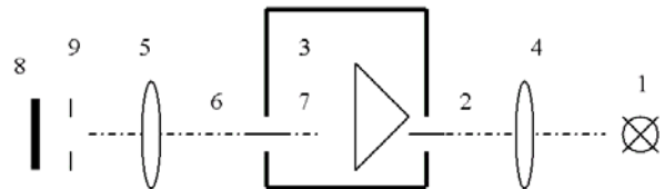
Fig.2 Optical diagram of measuring unit
