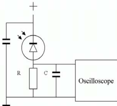
Fig.1 Calibration circuit.
