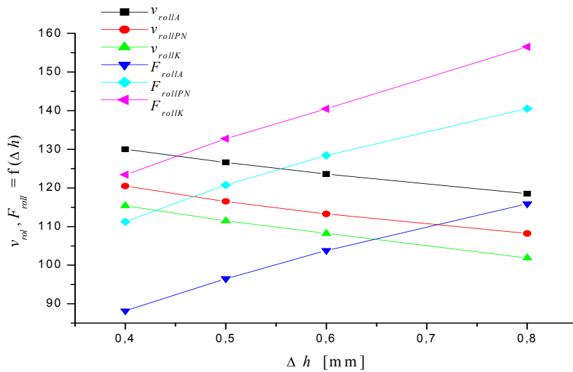
Fig.9. Theoretically determined rolling speed v_{\text{roll}} , rolling force F_{\text{roll}} for selected reductions \Delta h in relation to materials.
